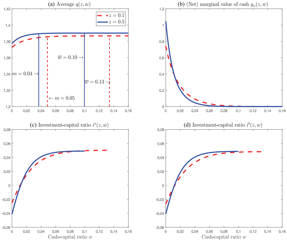
Figure 3. Refinancing case—comparison of diversified firms with z = 0.1 and z = 0.5 . In Panel A, the vertical lines mark the optimal payout boundary \bar{w} and the equity issuance amount m . (Color figure can be viewed at wileyonlinelibrary.com )
