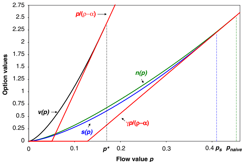
Fig. 2. The impact of time-inconsistent preferences on the option to wait for the case of flow payoffs. For the case of flow payoffs, this graph plots the option values of the time-consistent, naive, and sophisticated entrepreneurs, denoted as v(p) , n(p) , and s(p) , respectively. For the time-consistent entrepreneur, the investment payoff value is p/(\rho - \alpha) - I , while for the naive and sophisticated entrepreneurs the investment payoff value is \gamma p/(\rho - \alpha) - I . The vertical distance between an option value and the investment payoff value represents the value of the option to wait. The parameter values are \rho = 0.05 , \alpha = 0 , \sigma = 0.40 , \delta = 0.30 , \lambda = 0.33 , and I = 1 .
