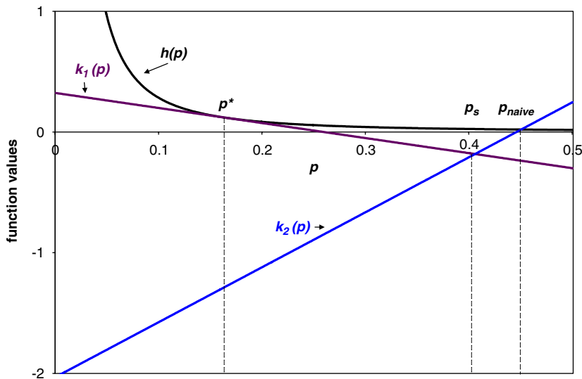
Fig. 3. Relative orderings of p^* , p_s , and p_{naive} . The curves k_1(p) and h(p) intersect (tangentially) at the point p^* . The curves k_1(p) and k_2(p) intersect at the point p_s , where we see that p_s > p^* . The curves k_2(p) and h(p) intersect at the point p_{naive} , where p_{naive} > p_s . The parameter values are \rho = 0.05 , \alpha = 0 , \sigma = 0.40 , \delta = 0.30 , \lambda = 0.33 , and I = 1 .
