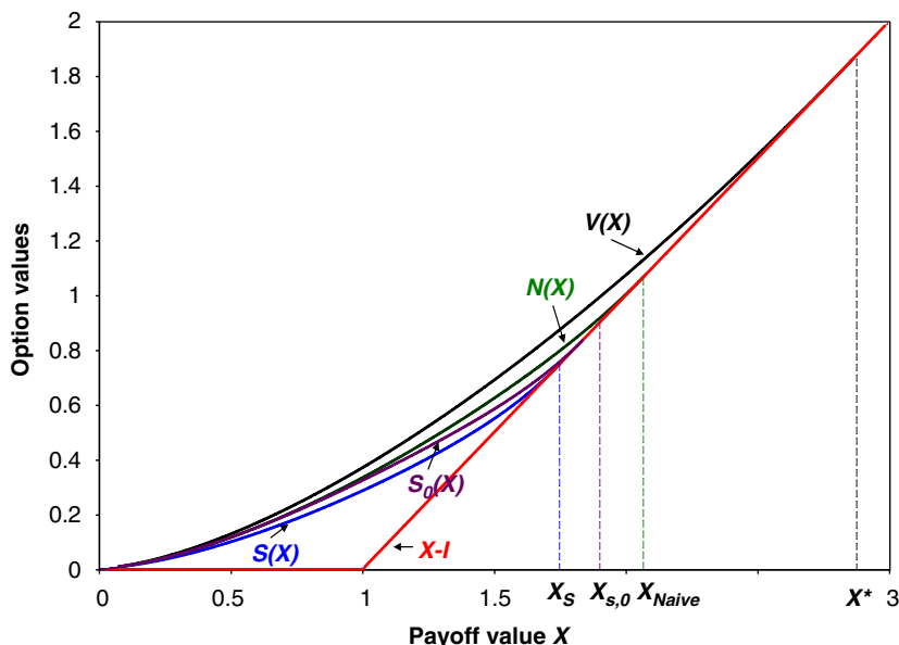
Fig. 1. The impact of time-inconsistent preferences on the option to wait. This graph plots the option values of the time-consistent, naive, sophisticated with a finite number of selves, and sophisticated with an infinite number of selves entrepreneurs, denoted as V(X) , N(X) , S_0(X) and S(X) , respectively. The vertical distance between an option value and the investment payoff value, X-I , represents the value of the option to wait. At all points prior to exercise, the time-consistent entrepreneur has the most valuable option to wait, followed by the naive entrepreneur, then the sophisticated entrepreneur with finite selves, and finally the sophisticated investor with an infinite number of selves. The parameter values are \rho = 0.05 , \alpha = 0 , \sigma = 0.35 , \delta = 0.90 , \lambda = 5 , I = 1 , and N = 5 for the sophisticated entrepreneur with finite selves.
